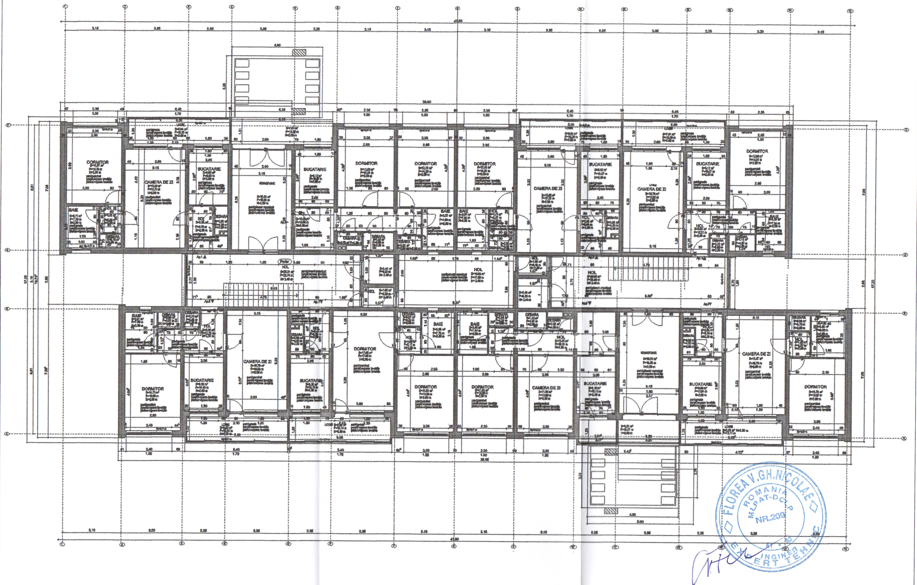
PLAN PARTER
