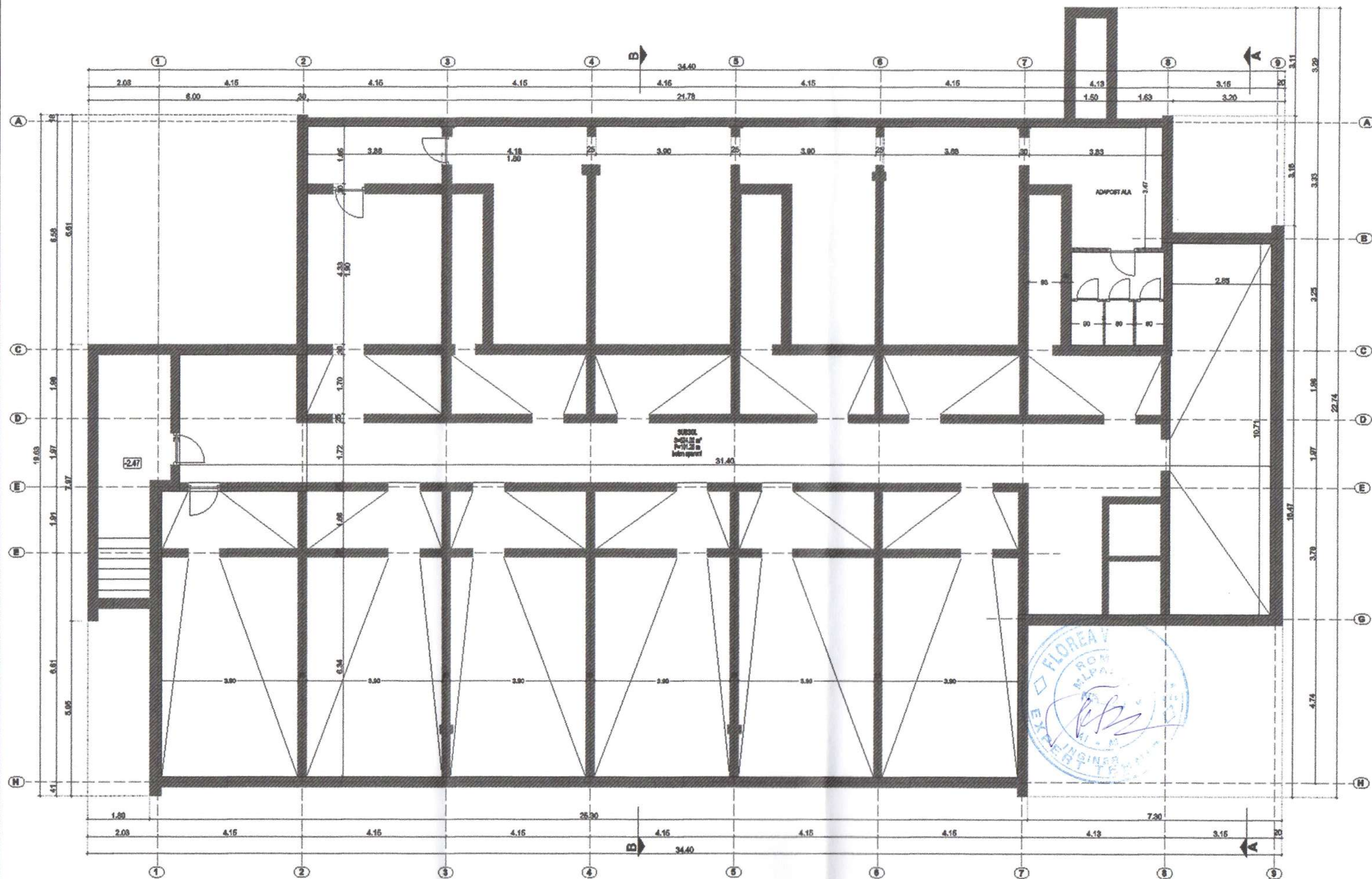
PLAN SUBSOL
